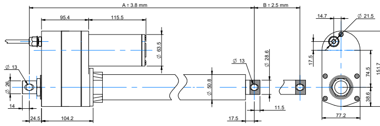
DRAWING (mm)
