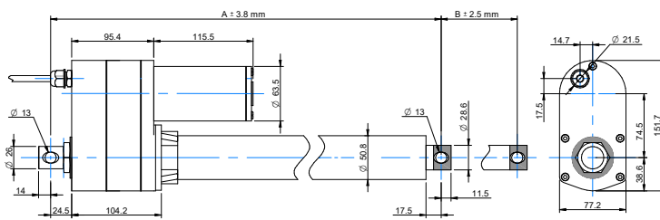
DRAWING (mm)
